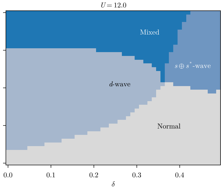
SC and normal regions ( t = 1.0 , L = 256 , \beta = 100.0 )
