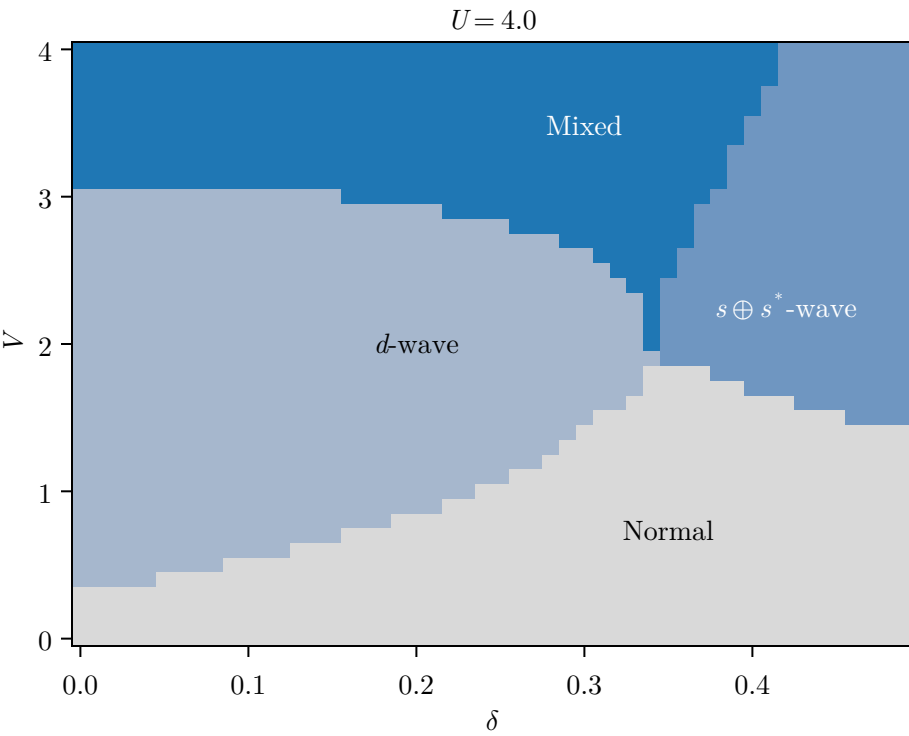
SC and normal regions ( t = 1.0 , L = 256 , \beta = 100.0 )
